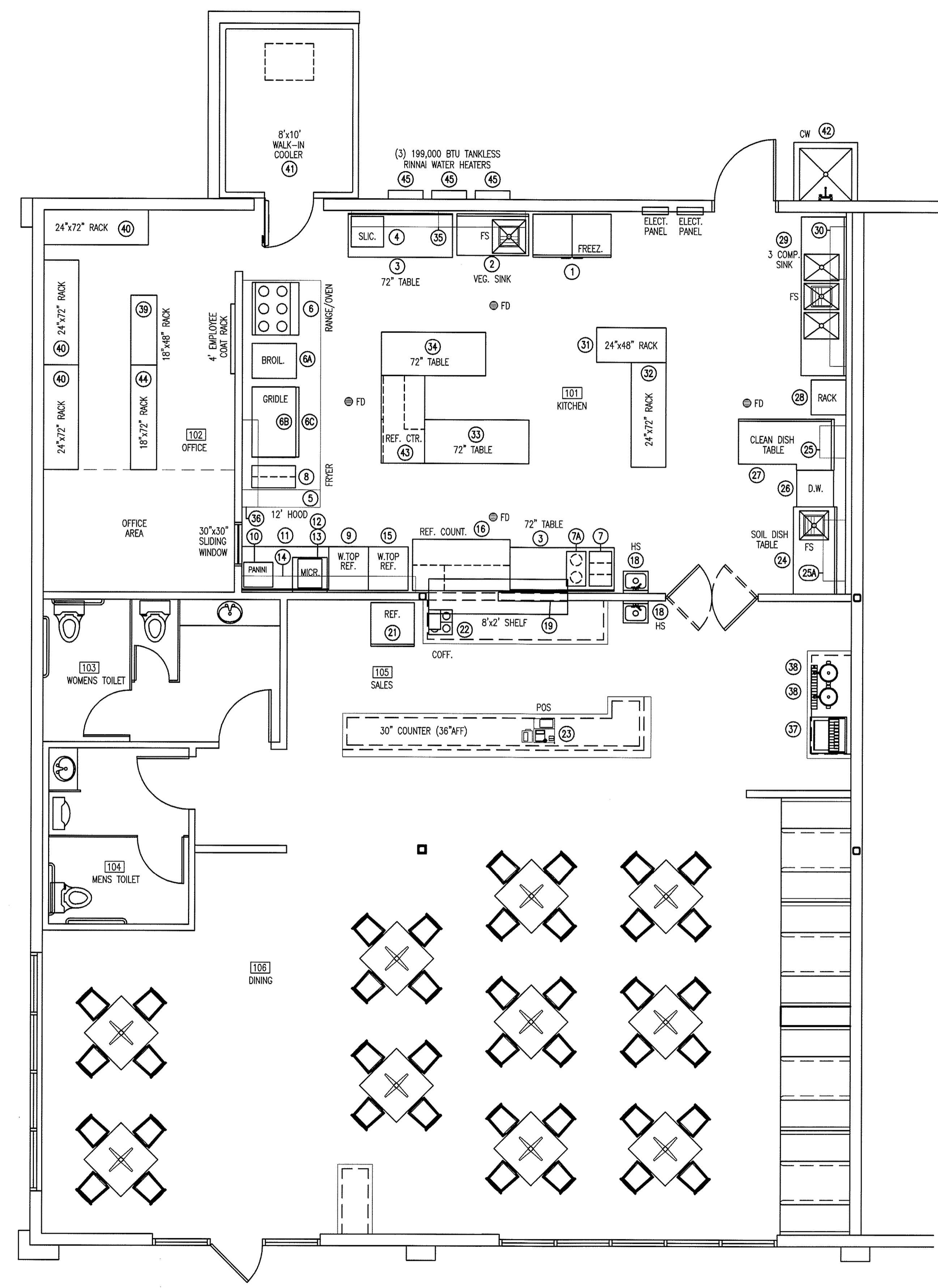
1 EQUIPMENT PLAN EQ-1 SCALE: 1/4" = 1'-0"
